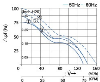
Performance FK 5523 ....
