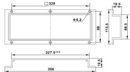
Drawing FK 6627.300
