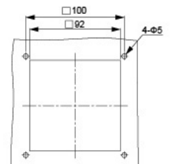
Drawing FKL 6621....
