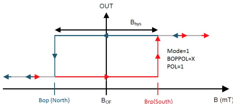
Latch: output voltage characteristic (Mode=1, BOPPOL=X, POL=1)
