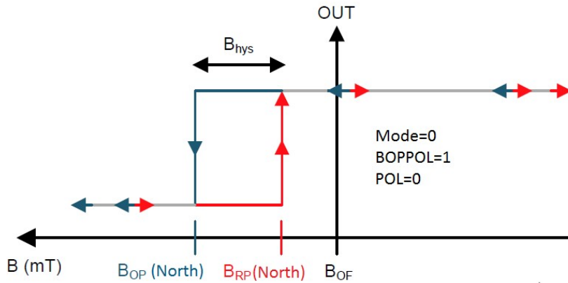
Unipolar: output voltage characteristic (Mode=0, BOPPOL=1, POL=0)
