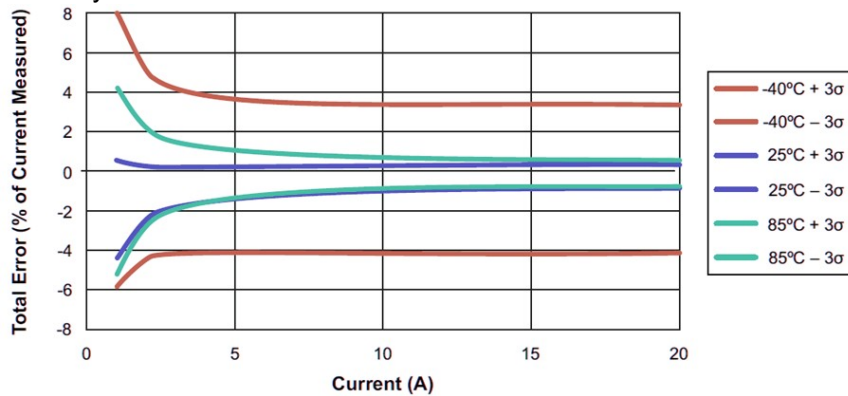
Figure 1: Predicted Total Error as a Function of the Sensed Current for the HC70120AB
