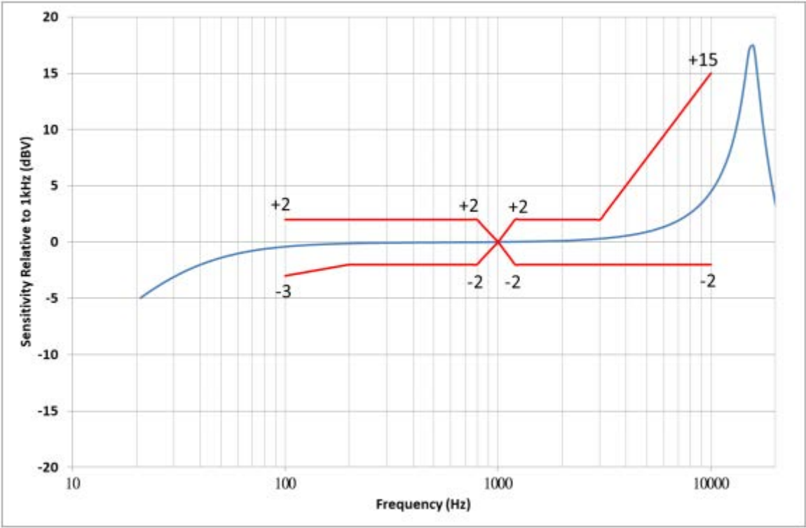
Typical frequency response normalized to 1KHz (Measured)
