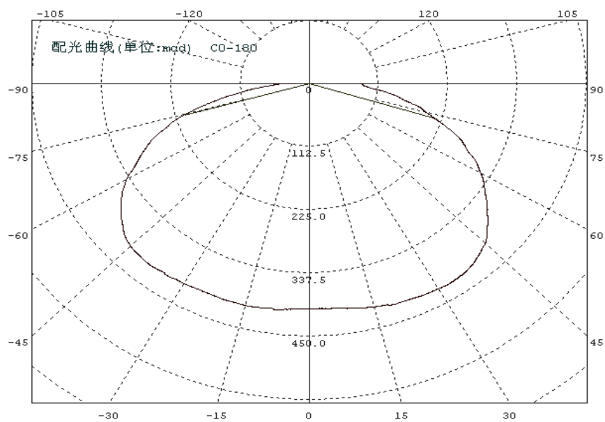
Directive Characteristics
