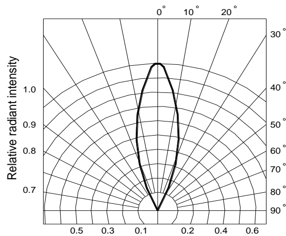
Fig.6 Radiation diagram
