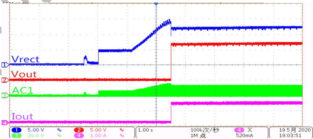
Figure 8. Transient Resp:CV8085D@Vout = 12V, Start up with 1.25A load
