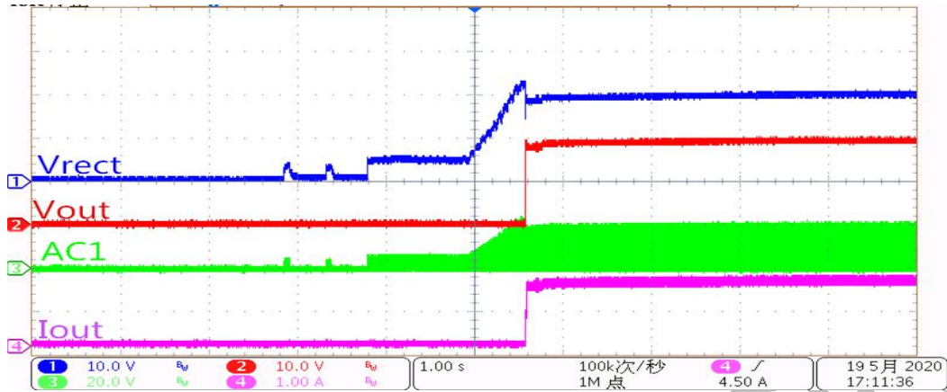
Figure 9. Transient Resp:CV8085D@Vout = 20V, Start up with 1.5A load
