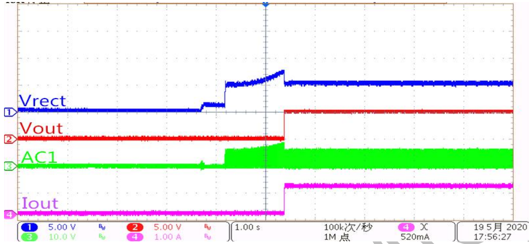
Figure 6. Transient Resp:CV8085D@Vout = 5V, Start up with 1A load
