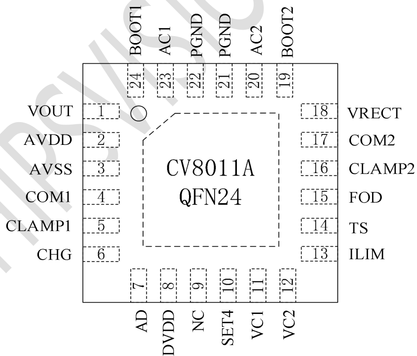
CV8011A Pin Diagram
