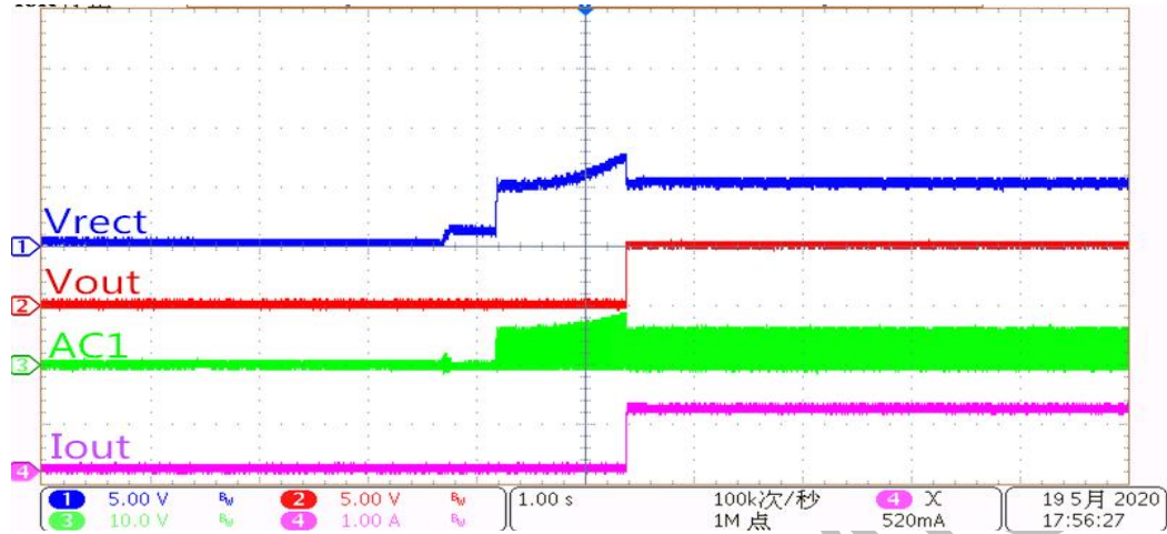
Figure 6. Transient Resp:CV8045D@ V_{out} = 5V , Start up with 1A load
