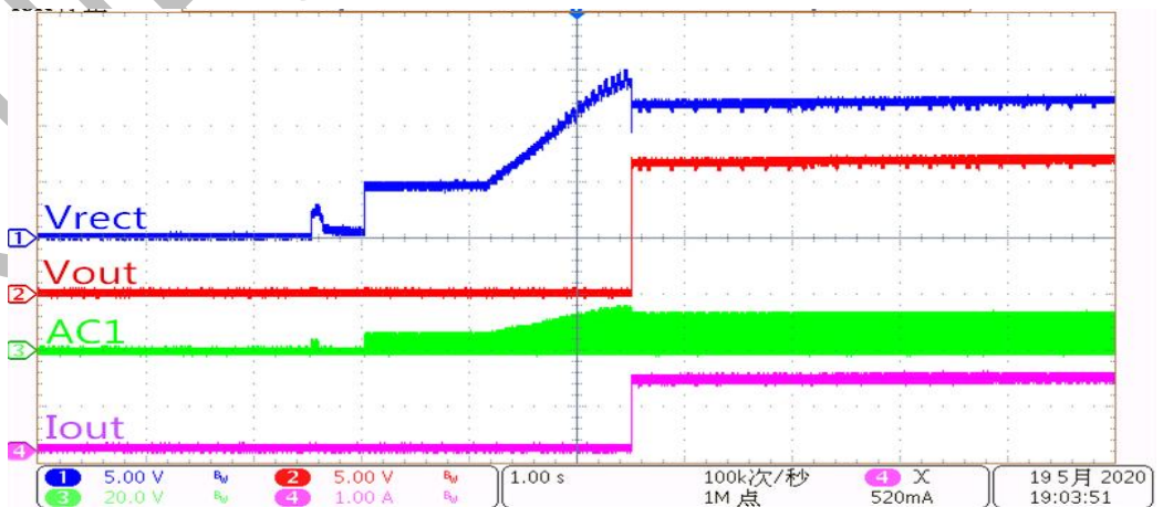
Figure 8. Transient Resp:CV8045D@ V_{out} = 12V , Start up with 1.25A load
