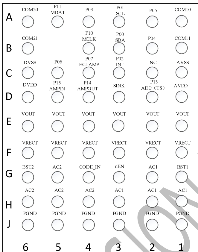
Bottom View
