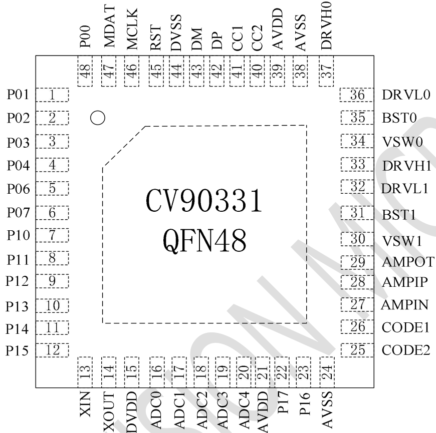
Figure 2 CV90331引脚图
