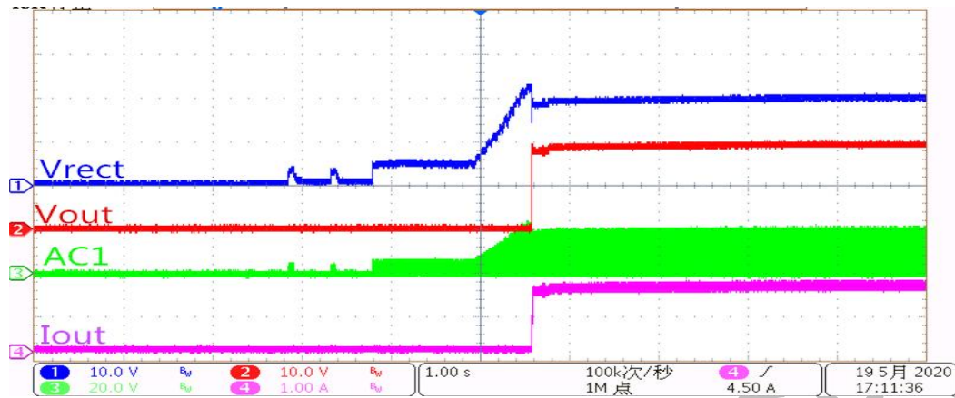
Figure 9. Transient Resp:CV8055D@Vout = 20V, Start up with 1.5A load
