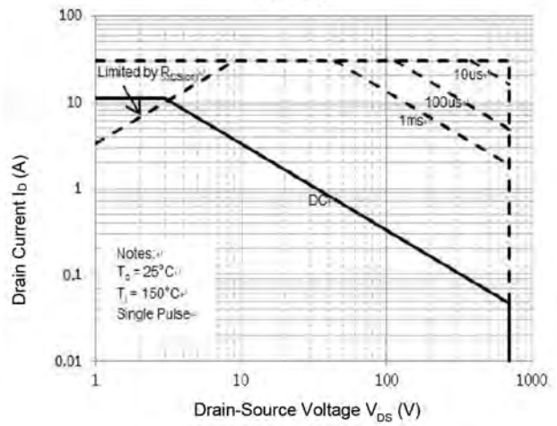
Figure 10. Maximum Safe Operating Area TO-220F
