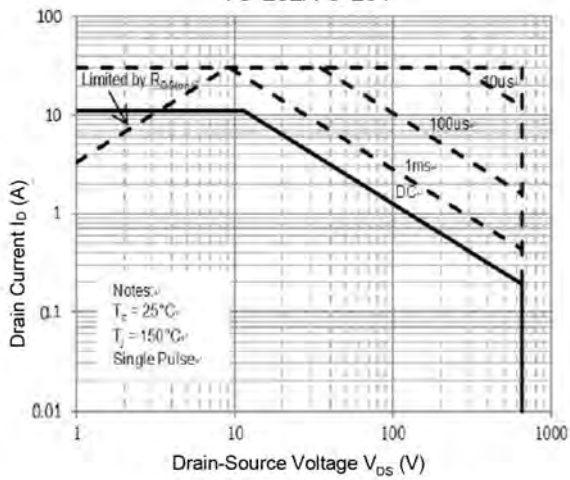
Figure 9. Maximum Safe Operating Area TO-252/TO-251
