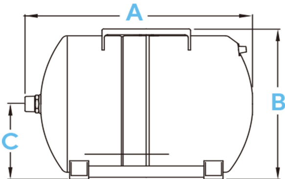
卧式8L~100L
