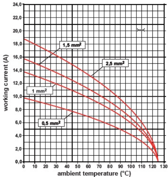
Derating curves
