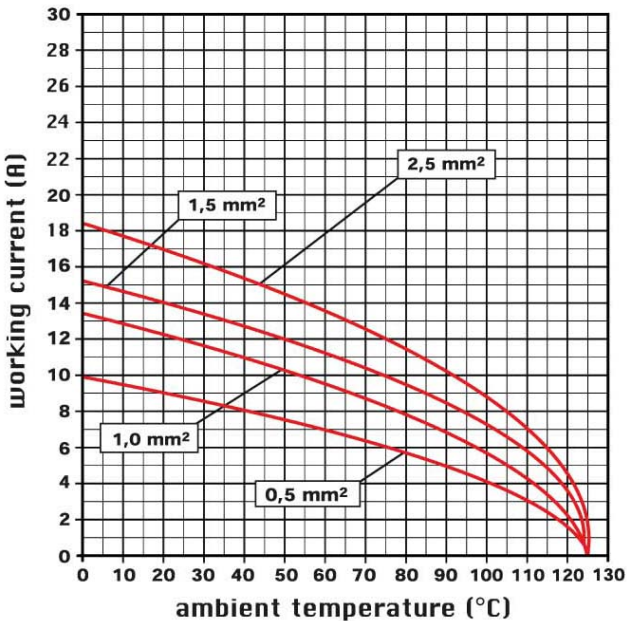
diagram CSH 24 poles
