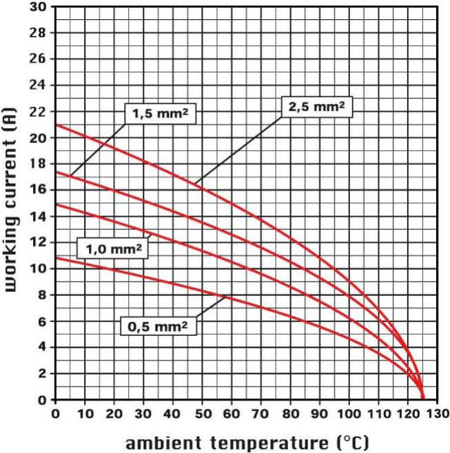
diagram CSH 16 poles
