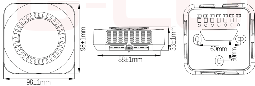
AQ22.XX/AQT22.XX
