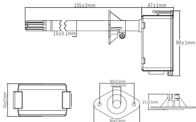
AQ32.XX/AQT32.XX
