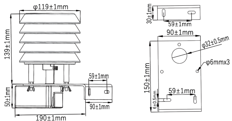
AQ32.XX/AQT32.XX
