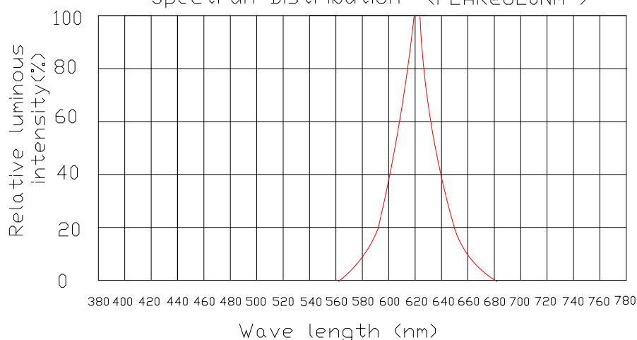
Spectrum Distribution (PEAK@620NM )
