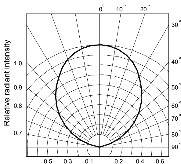
Fig.6 Radiation diagram
