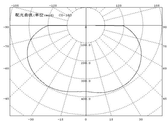
Directive Characteristics
