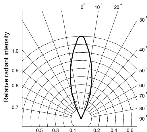
Fig.6 Radiation diagram
