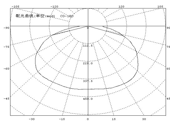
Directive Characteristics
