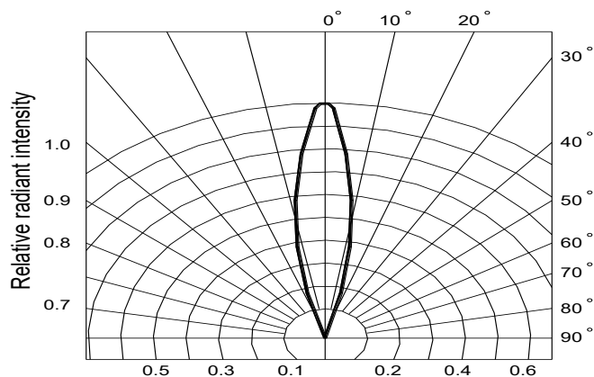
Fig.6 Radiation diagram
