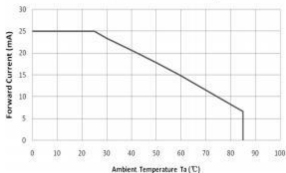
Maximum Forward Current VS. Ambient temperature
