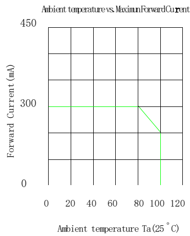
Detrating
