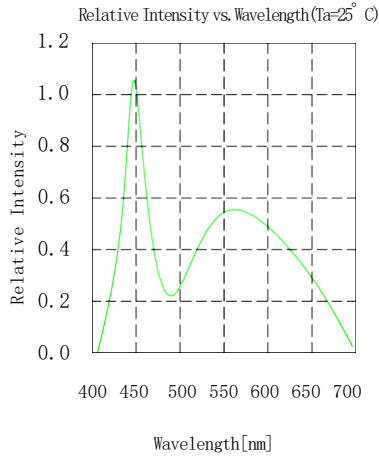
Spectral Distribution
