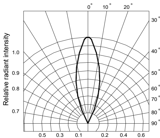
Fig.6 Radiation diagram
