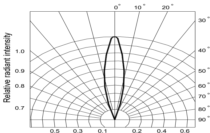
Fig.6 Radiation diagram
