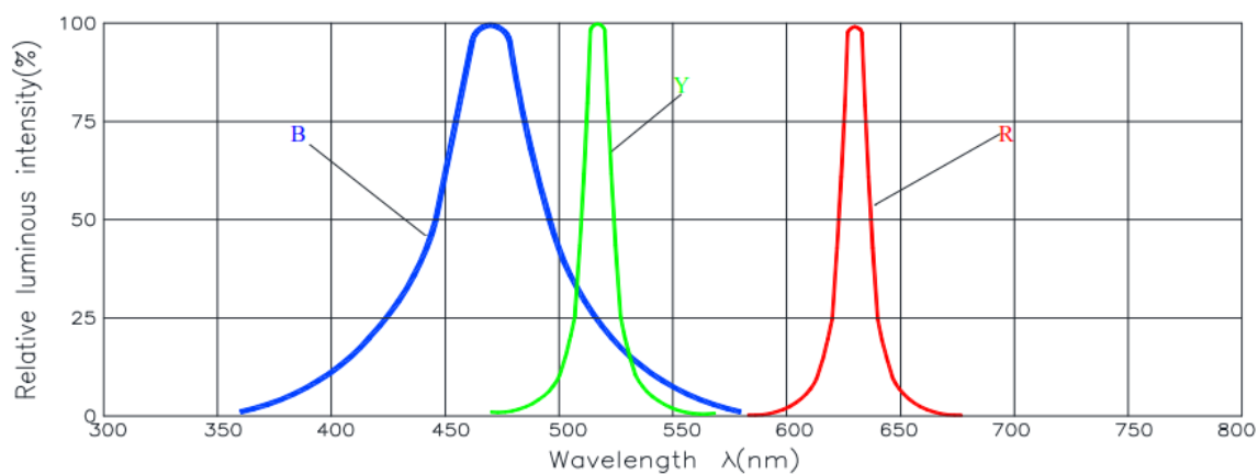
Spectrum Distribution
