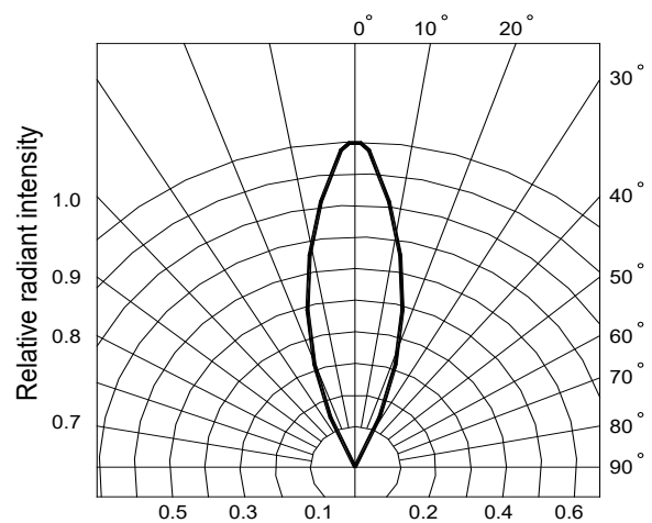
Fig.6 Radiation diagram
