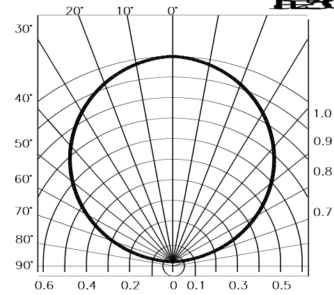
Beam Angle vs. Relative luminous intensity
