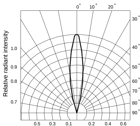
Fig.6 Radiation diagram
