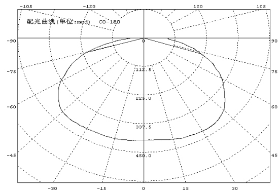
Directive Characteristics
