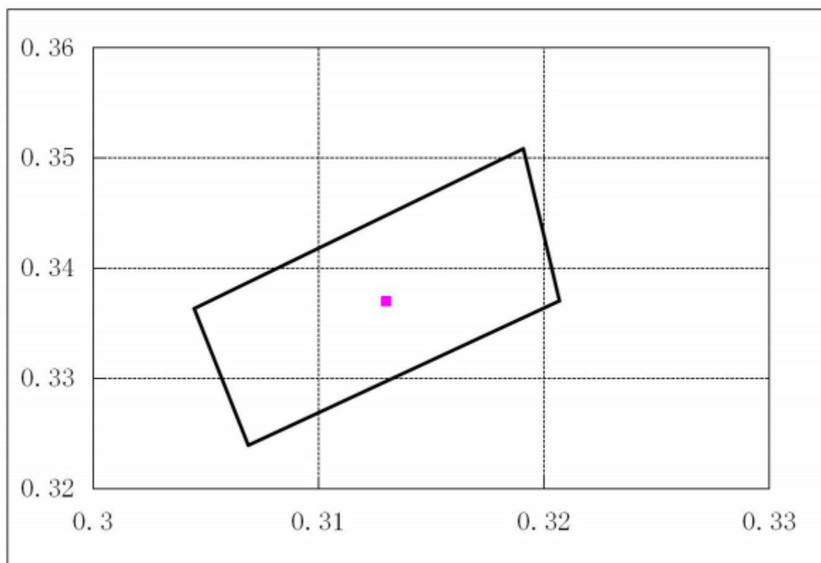
CIE Chromaticity Diagram CIE 色度图
