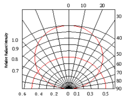
Relative Radiant Intensity VS. Angular Displacement
