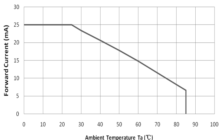
Maximum Forward Current VS. Ambient temperature
