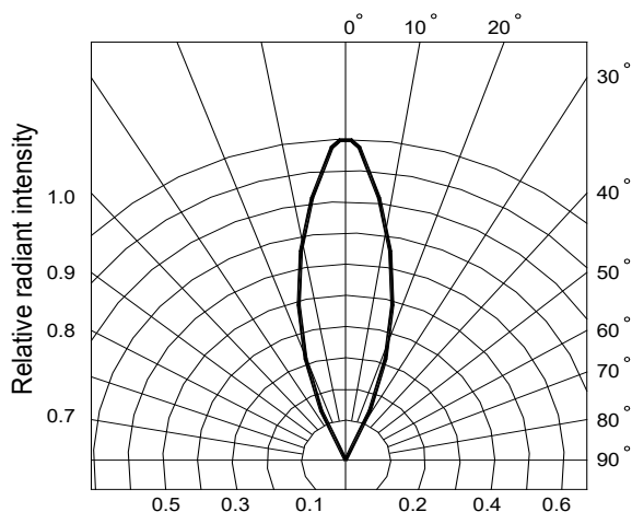
Fig.6 Radiation diagram
