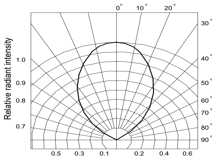
Fig.6 Radiation diagram
