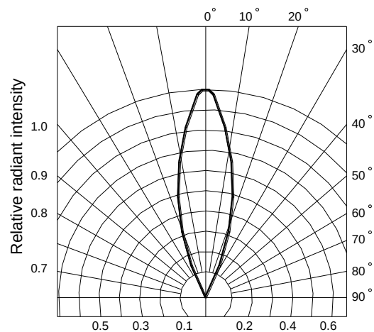
Fig.6 Radiation diagram
