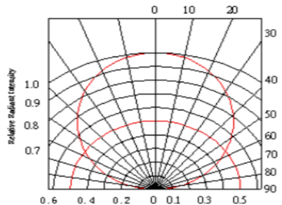
Relative Radiant Intensity VS. Angular Displacement 辐射强度与角度关系曲线图
