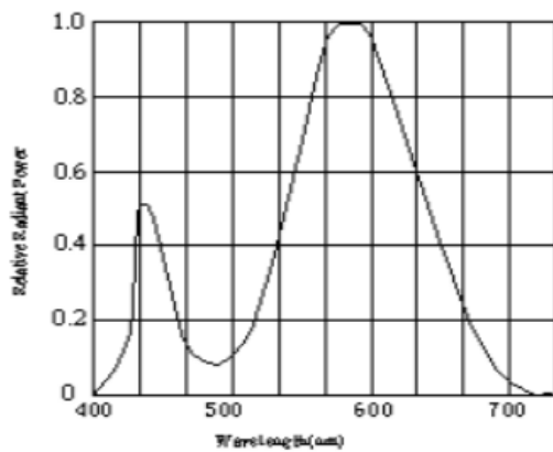
Relative Radiant power VS. Wavelength 辐射功率与波长关系曲线图
