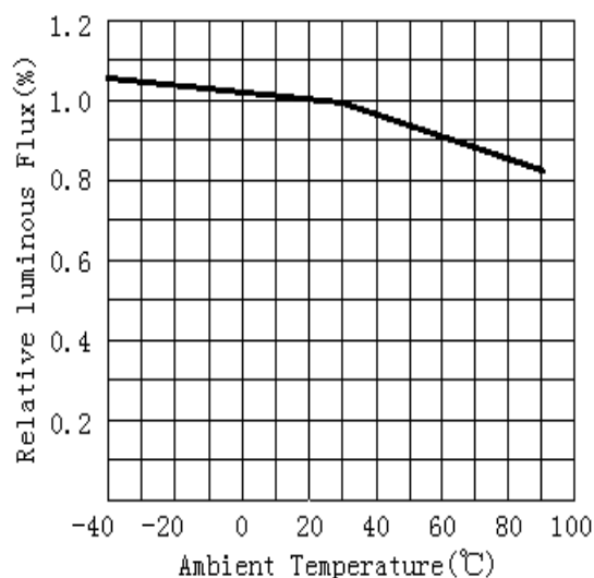
Relative Luminous Flux VS. Ambient Temperature 温度与亮度关系曲线图
