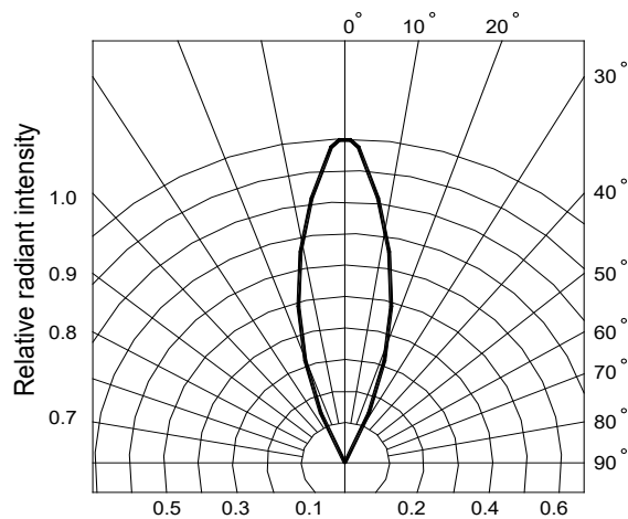
Fig.6 Radiation diagram
