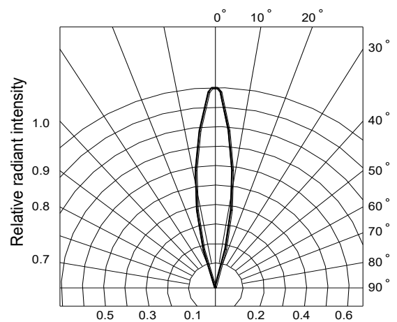
Fig.6 Radiation diagram
