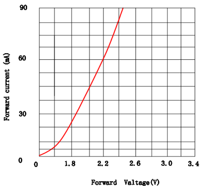
Forward Current VS. Forward Voltage 电压与电流关系曲线图
