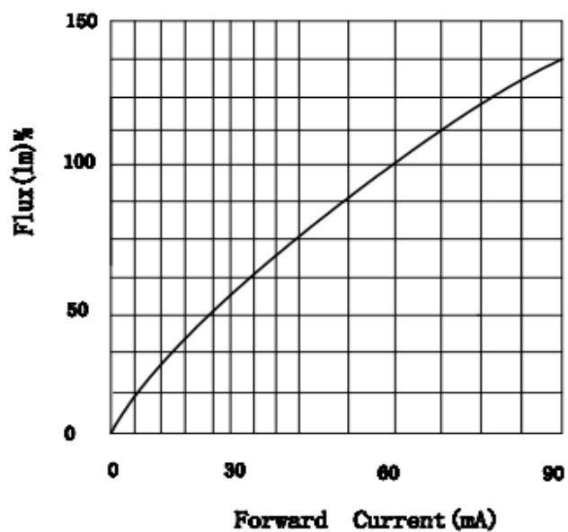
Relative Luminous Flux VS. Forward Current 亮度与电流关系曲线图
