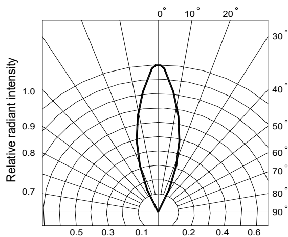
Fig.6 Radiation diagram
