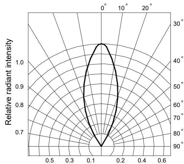
Fig.6 Radiation diagram
