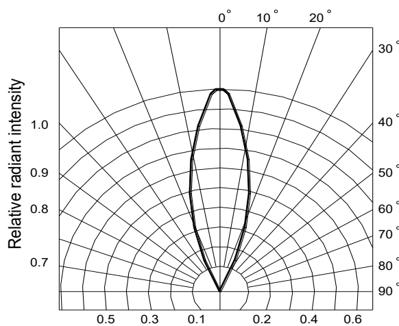
Fig.6 Radiation diagram
