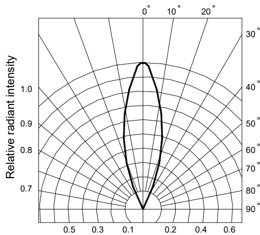
Fig.6 Radiation diagram
