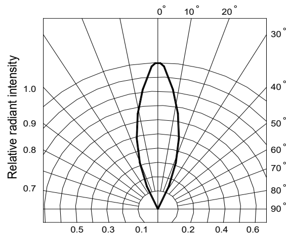
Fig.6 Radiation diagram
