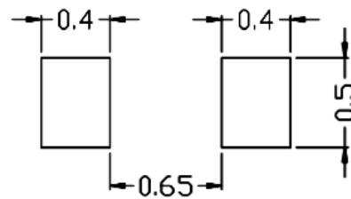
Recommend Pad Layout
