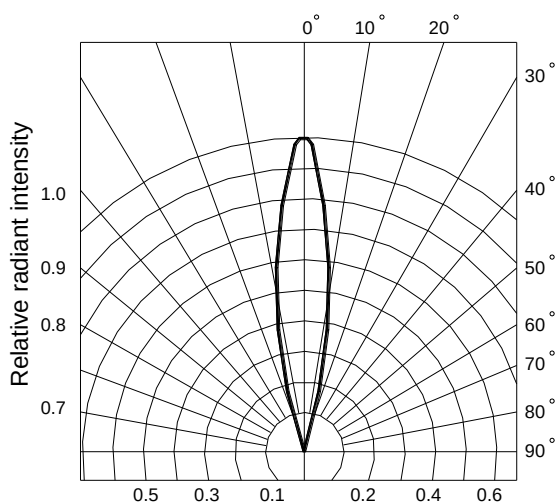
Fig.6 Radiation diagram
