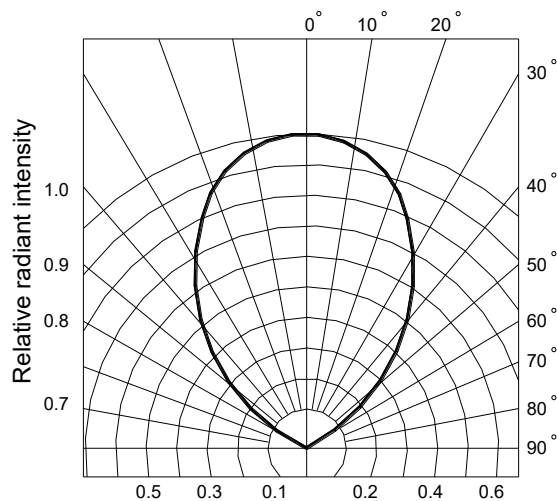
Fig.6 Radiation diagram
